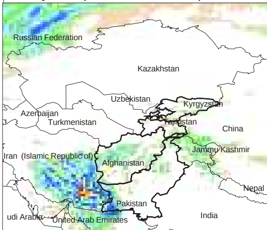
Daily Precip. Forecast for 7 Apr., 2013
