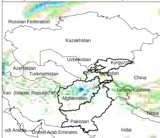
Daily Precip. Forecast for 11 Apr., 2013
