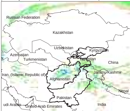
Daily Precip. Forecast for 10 Apr., 2013
