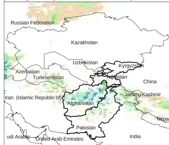
Daily Precip. Forecast for 12 Apr., 2013
