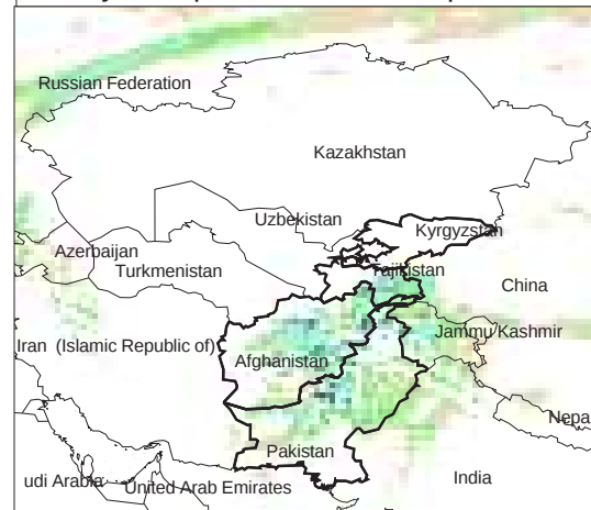
Daily Precip. Forecast for 9 Apr., 2013
