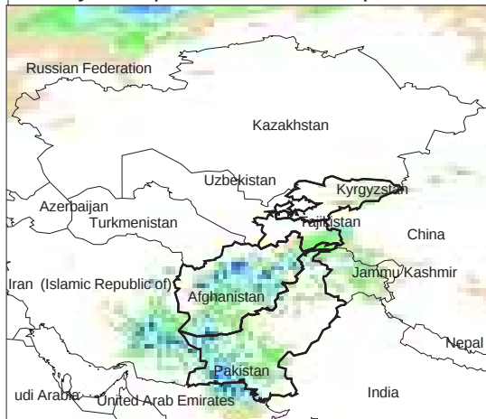
Daily Precip. Forecast for 8 Apr., 2013
