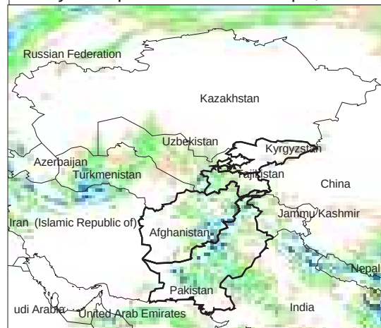
Daily Precip. Forecast for 22 Apr., 2013
