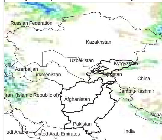
Daily Precip. Forecast for 16 May, 2013
