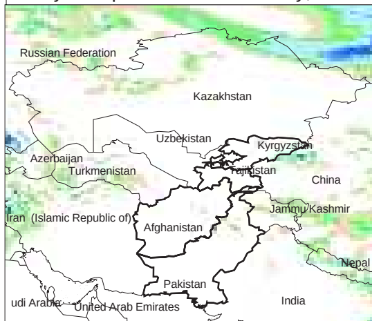
Daily Precip. Forecast for 15 May, 2013
