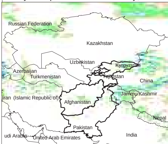
Daily Precip. Forecast for 14 May, 2013
