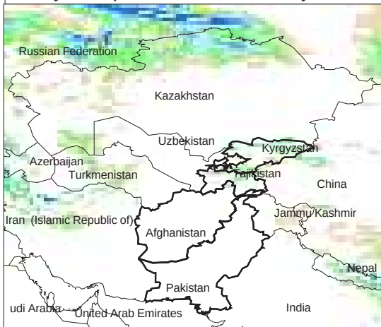
Daily Precip. Forecast for 17 May, 2013
