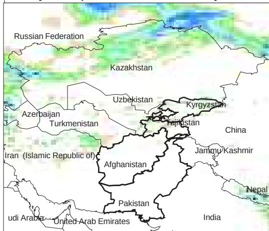
Daily Precip. Forecast for 18 May, 2013
