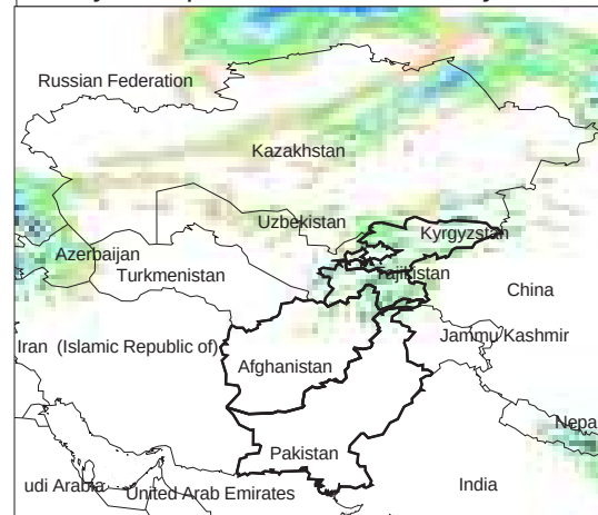
Daily Precip. Forecast for 19 May, 2013
