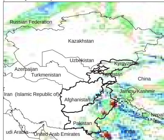
Daily Precip. Forecast for 14 Jun., 2013
