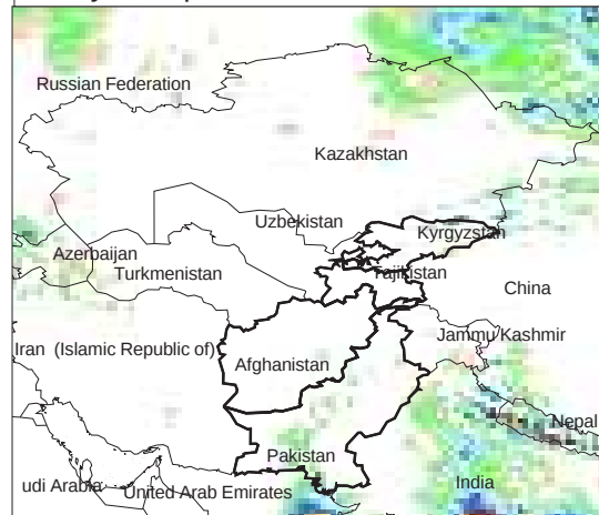
Daily Precip. Forecast for 11 Jun., 2013
