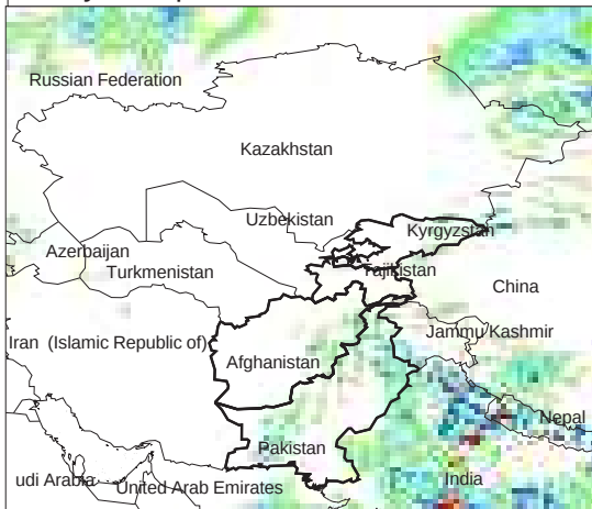
Daily Precip. Forecast for 12 Jun., 2013
