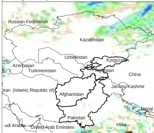
Daily Precip. Forecast for 10 Jun., 2013
