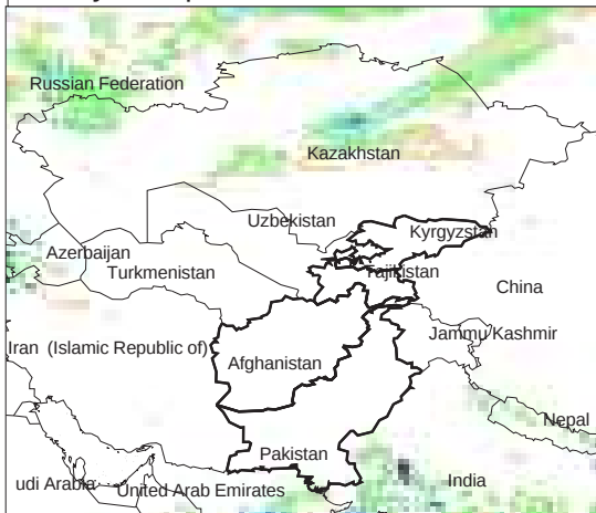
Daily Precip. Forecast for 9 Jun., 2013
