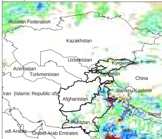
Daily Precip. Forecast for 13 Jun., 2013
