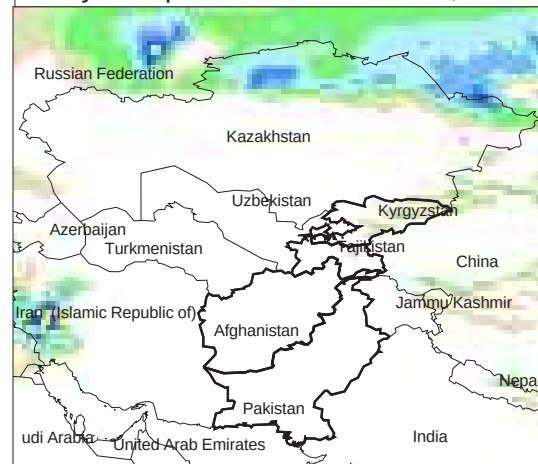
Daily Precip. Forecast for 13 Dec., 2013
