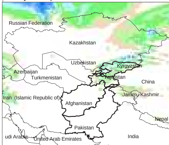
Daily Precip. Forecast for 12 Dec., 2013
