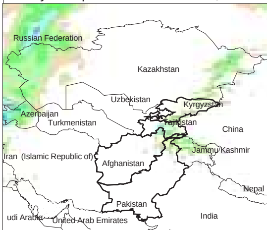
Daily Precip. Forecast for 8 Dec., 2013
