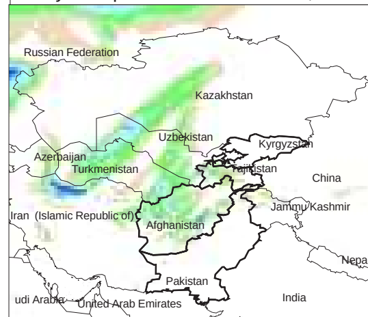
Daily Precip. Forecast for 10 Dec., 2013
