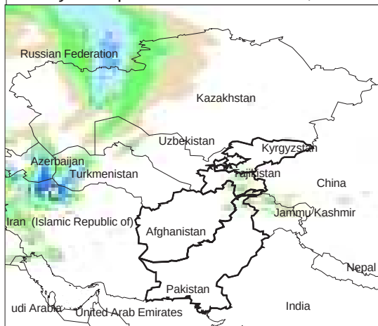
Daily Precip. Forecast for 9 Dec., 2013
