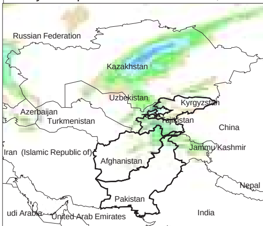
Daily Precip. Forecast for 11 Dec., 2013
