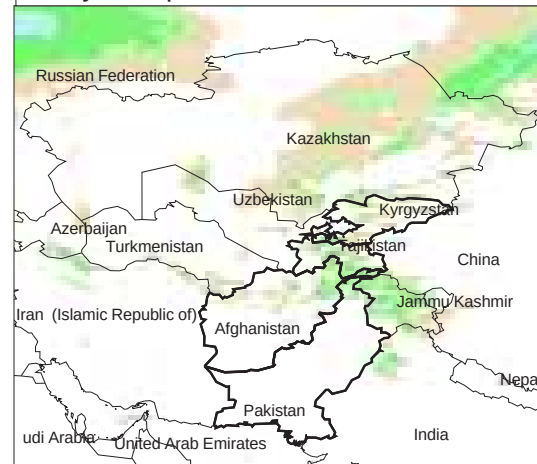
Daily Precip. Forecast for 21 Dec., 2013
