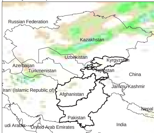
Daily Precip. Forecast for 20 Dec., 2013
