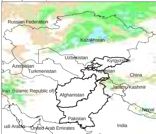
Daily Precip. Forecast for 19 Dec., 2013
