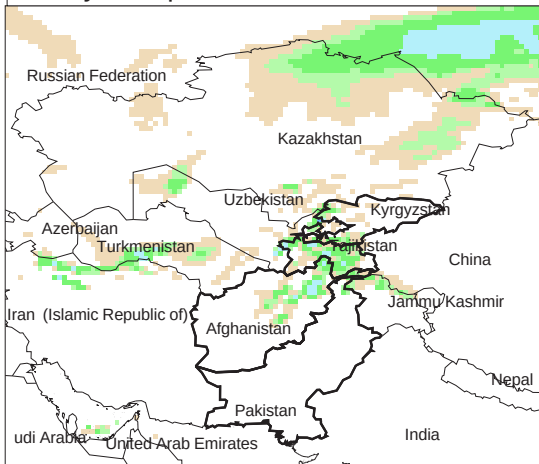
Daily Precip. Forecast for 3 Jan., 2014
