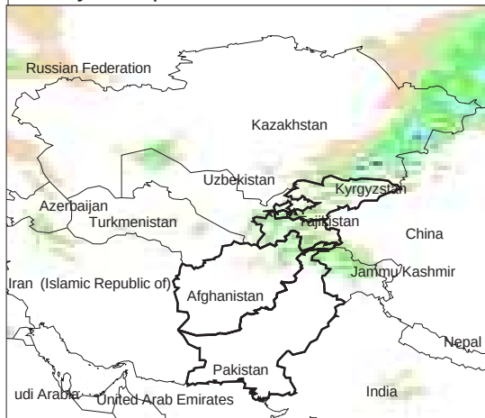
Daily Precip. Forecast for 4 Jan., 2014
