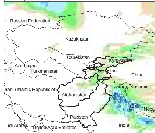
Daily Precip. Forecast for 14 Feb., 2014
