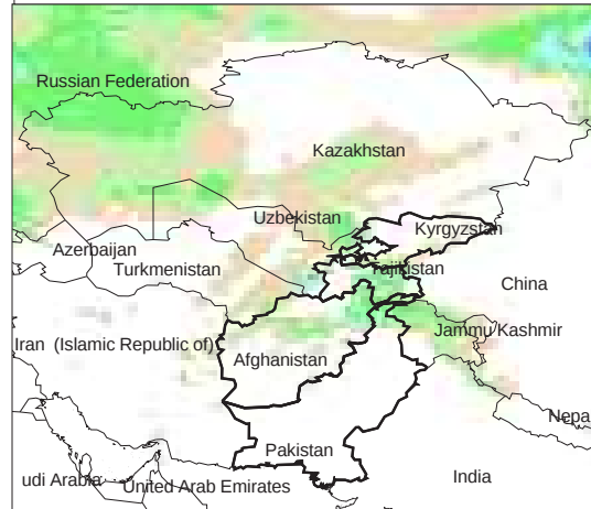
Daily Precip. Forecast for 18 Feb., 2014
