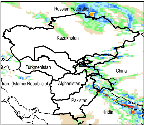
Daily Precip. Forecast for 2 Jul., 2014
