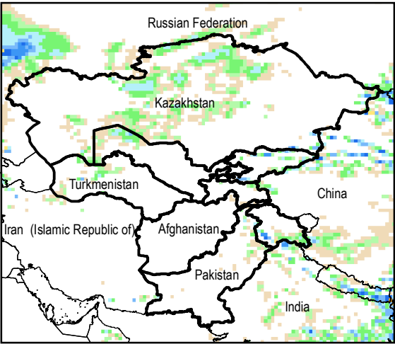
Daily Precip. Forecast for 30 Jun., 2014
