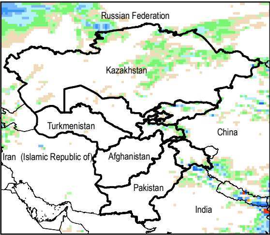
Daily Precip. Forecast for 1 Jul., 2014
