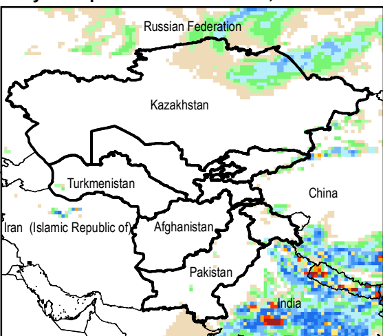
Daily Precip. Forecast for 15 Jul., 2014
