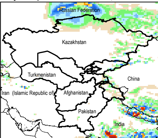
Daily Precip. Forecast for 16 Jul., 2014
