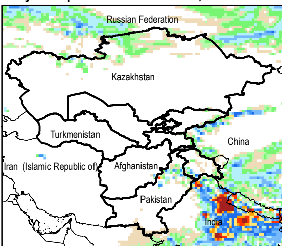
Daily Precip. Forecast for 17 Jul., 2014
