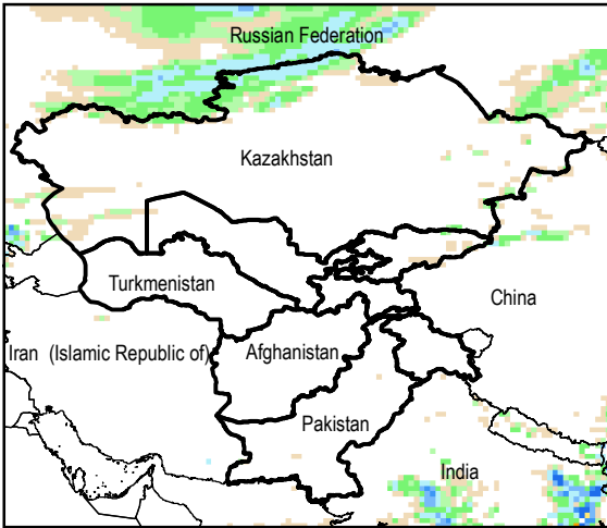
Daily Precip. Forecast for 19 Sep., 2014
