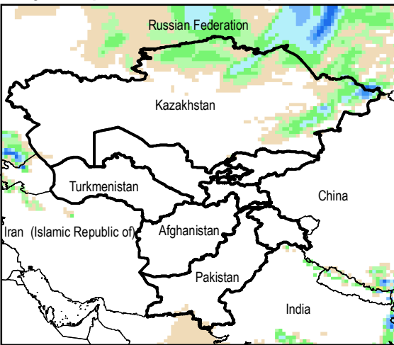
Daily Precip. Forecast for 18 Sep., 2014
