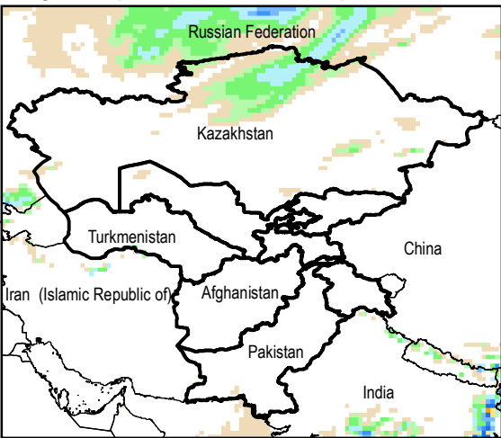
Daily Precip. Forecast for 17 Sep., 2014
