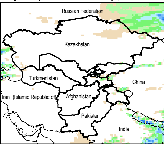
Daily Precip. Forecast for 20 Sep., 2014
