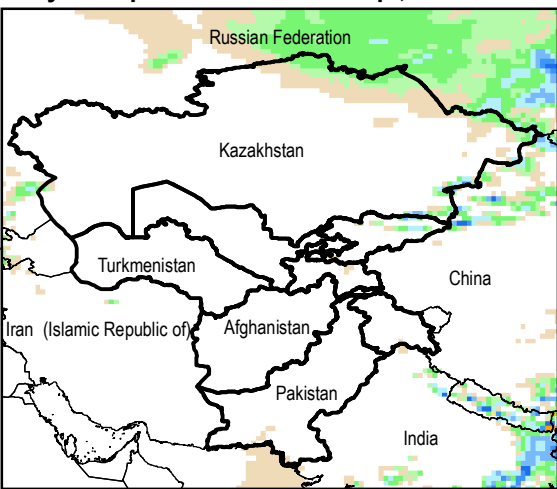
Daily Precip. Forecast for 19 Sep., 2014
