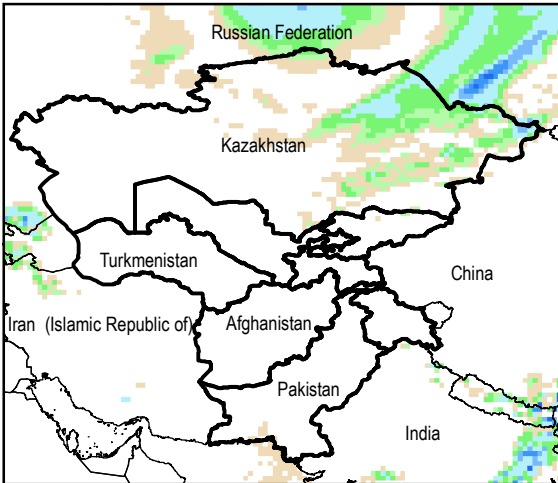
Daily Precip. Forecast for 21 Sep., 2014
