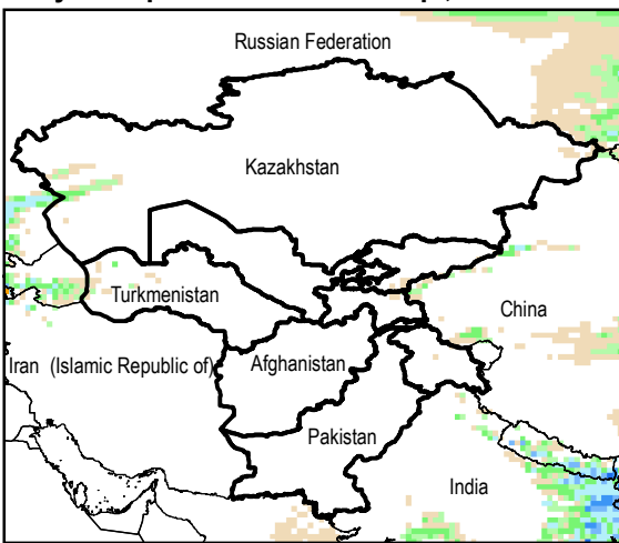
Daily Precip. Forecast for 21 Sep., 2014
