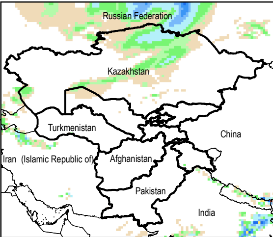
Daily Precip. Forecast for 20 Sep., 2014
