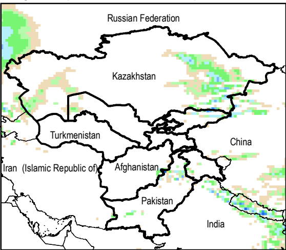
Daily Precip. Forecast for 25 Sep., 2014
