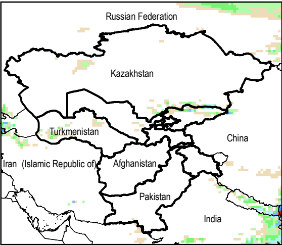
Daily Precip. Forecast for 25 Sep., 2014
