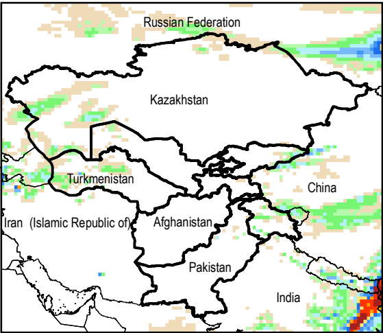
Daily Precip. Forecast for 24 Sep., 2014
