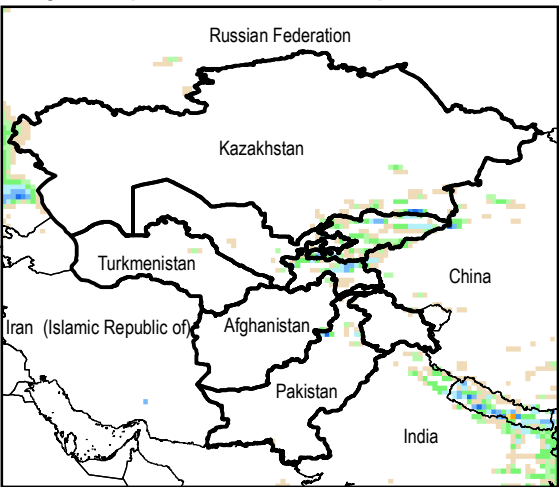
Daily Precip. Forecast for 24 Sep., 2014
