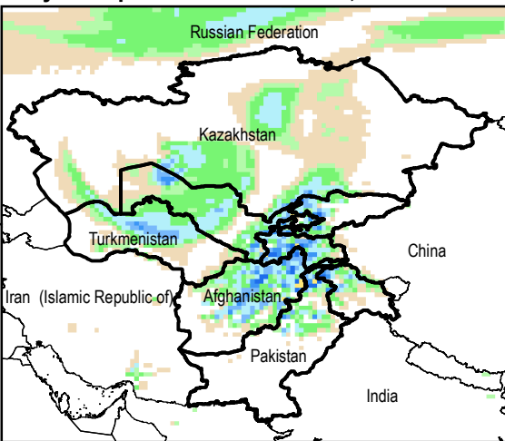
Daily Precip. Forecast for 9 Nov., 2014
