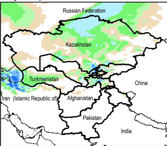
Daily Precip. Forecast for 6 Dec., 2014
