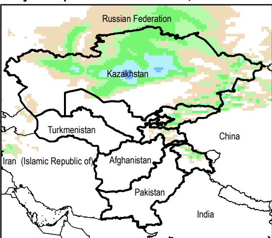
Daily Precip. Forecast for 5 Dec., 2014
