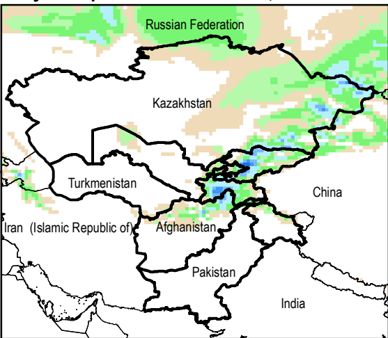
Daily Precip. Forecast for 10 Dec., 2014
