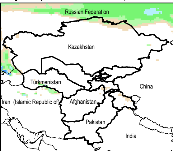
Daily Precip. Forecast for 11 Dec., 2014
