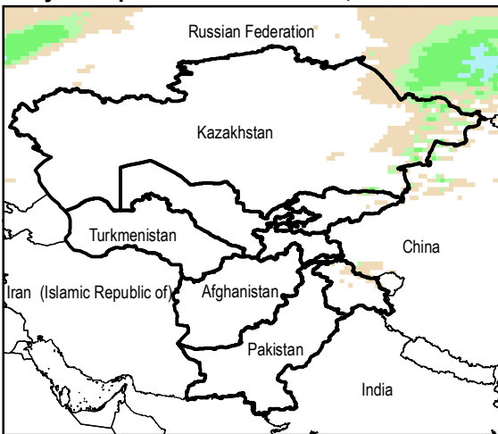
Daily Precip. Forecast for 12 Dec., 2014
