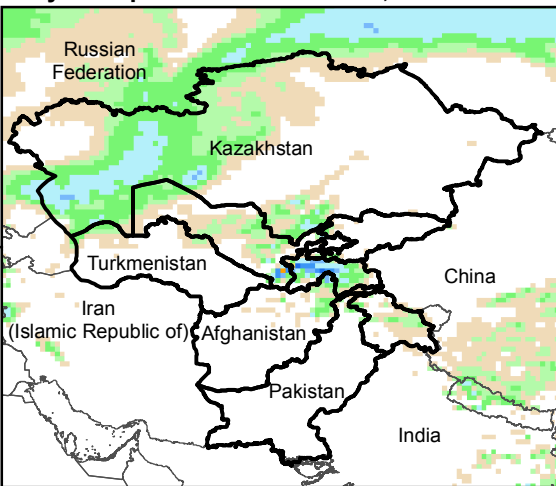
Daily Precip. Forecast for 7 Jan., 2015
