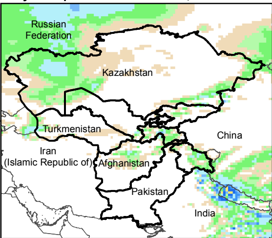
Daily Precip. Forecast for 6 Jan., 2015
