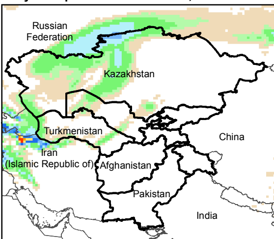
Daily Precip. Forecast for 8 Jan., 2015
