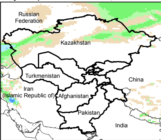
Daily Precip. Forecast for 10 Jan., 2015
