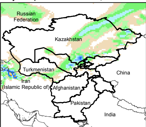
Daily Precip. Forecast for 9 Jan., 2015
