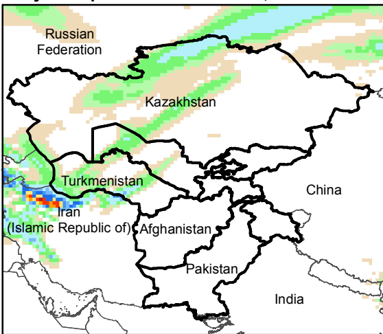
Daily Precip. Forecast for 11 Jan., 2015
