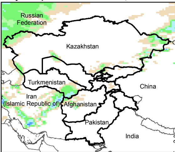
Daily Precip. Forecast for 13 Jan., 2015
