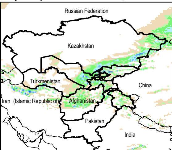
Daily Precip. Forecast for 26 Jan., 2015
