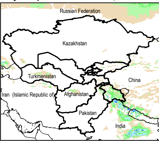
Daily Precip. Forecast for 27 Jan., 2015
