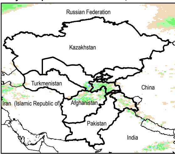
Daily Precip. Forecast for 28 Jan., 2015
