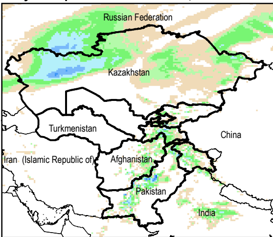
Daily Precip. Forecast for 10 Feb., 2015
