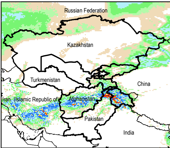
Daily Precip. Forecast for 19 Feb., 2015
