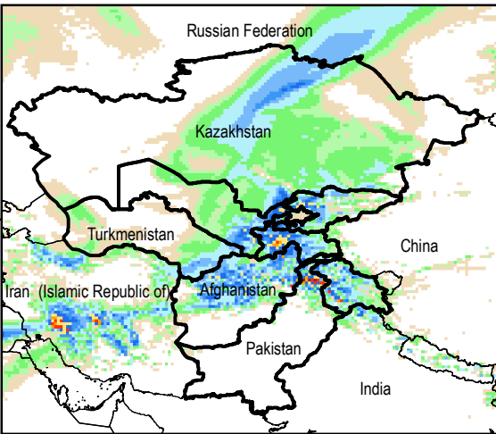
Daily Precip. Forecast for 18 Feb., 2015
