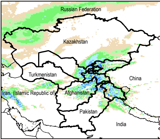
Daily Precip. Forecast for 19 Feb., 2015
