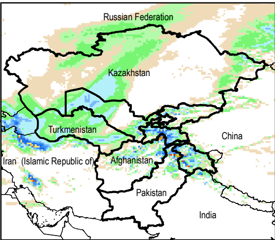
Daily Precip. Forecast for 17 Feb., 2015
