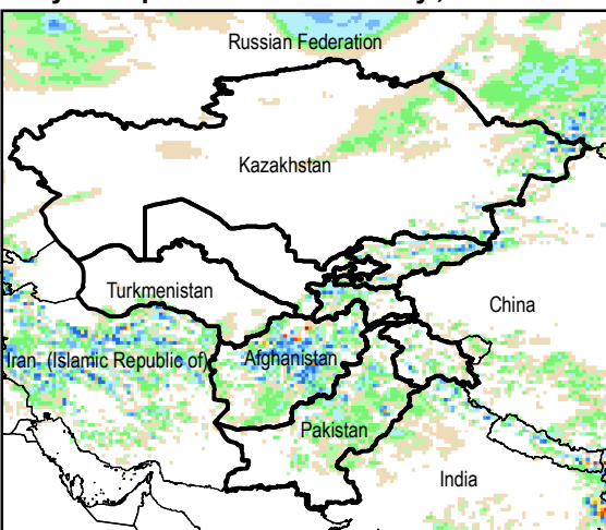
Daily Precip. Forecast for 10 May., 2015
