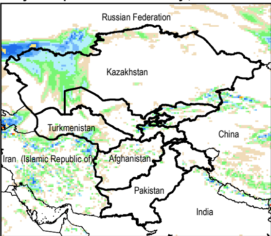
Daily Precip. Forecast for 9 May., 2015
