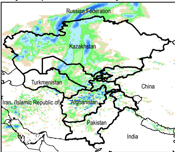
Daily Precip. Forecast for 11 May., 2015
