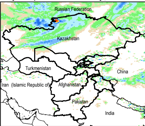
Daily Precip. Forecast for 22 May., 2015
