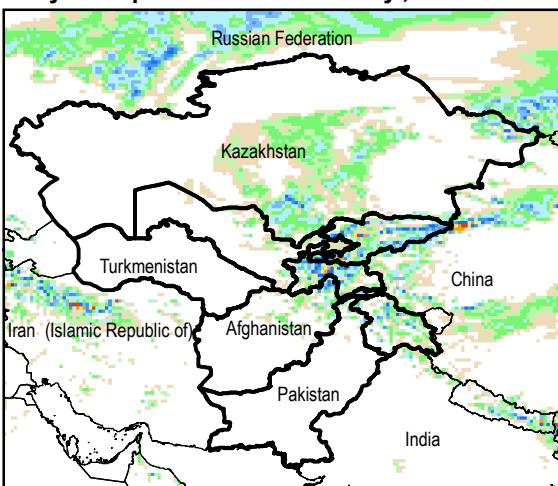
Daily Precip. Forecast for 23 May., 2015
