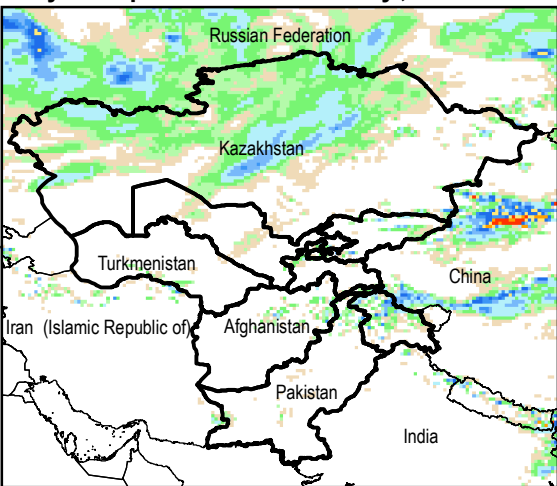
Daily Precip. Forecast for 21 May., 2015
