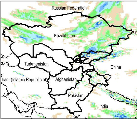
Daily Precip. Forecast for 6 Sep., 2015
