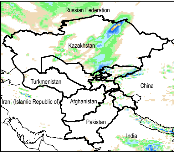
Daily Precip. Forecast for 5 Sep., 2015
