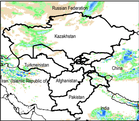
Daily Precip. Forecast for 4 Sep., 2015
