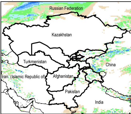
Daily Precip. Forecast for 6 Sep., 2015
