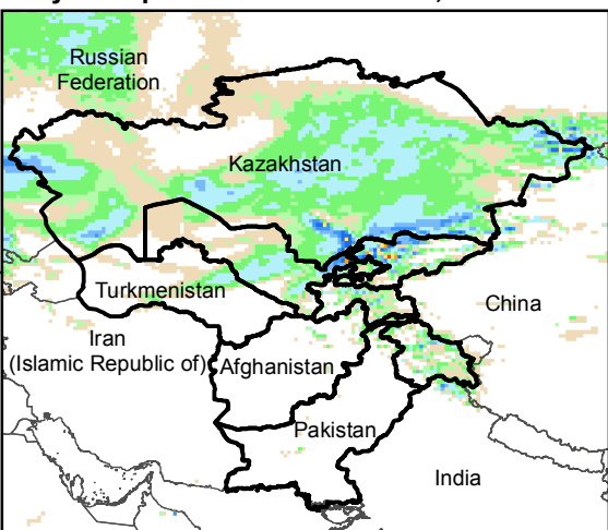
Daily Precip. Forecast for 13 Nov., 2015
