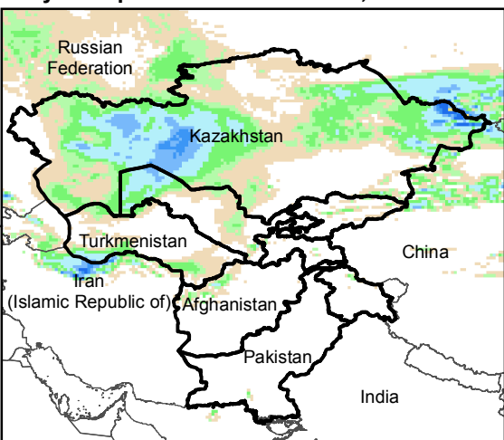
Daily Precip. Forecast for 14 Nov., 2015
