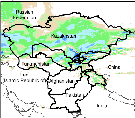
Daily Precip. Forecast for 16 Nov., 2015
