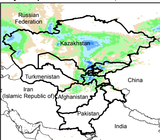
Daily Precip. Forecast for 15 Nov., 2015
