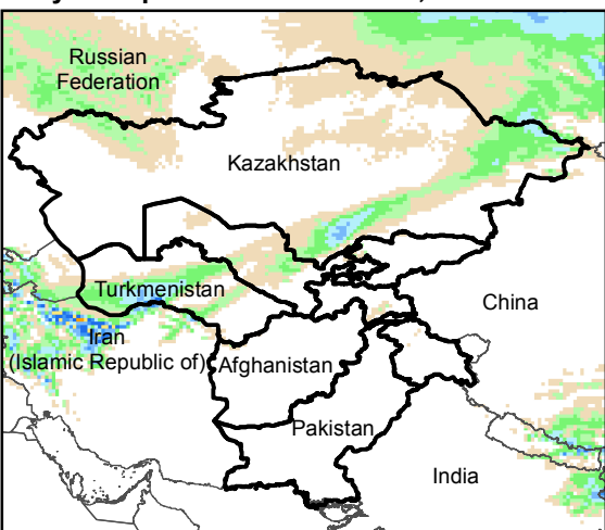
Daily Precip. Forecast for 8 Feb., 2016
