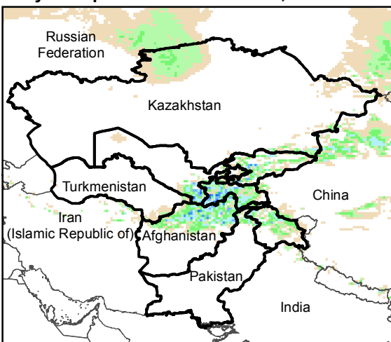
Daily Precip. Forecast for 10 Feb., 2016
