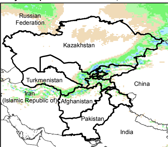
Daily Precip. Forecast for 9 Feb., 2016
