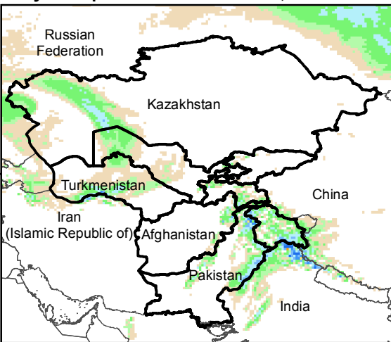
Daily Precip. Forecast for 22 Feb., 2016
