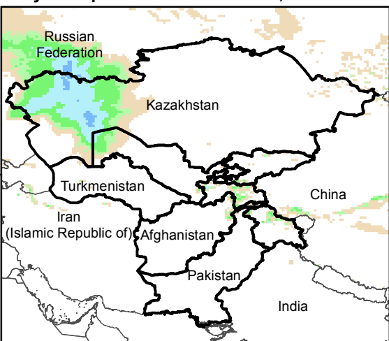
Daily Precip. Forecast for 21 Feb., 2016
