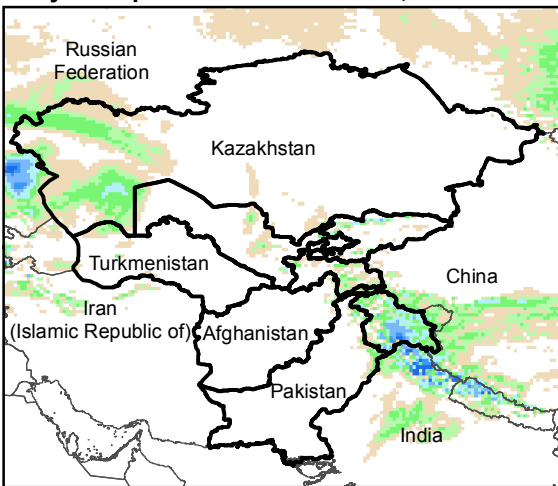
Daily Precip. Forecast for 23 Feb., 2016
