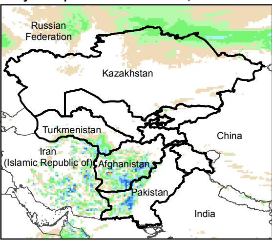
Daily Precip. Forecast for 1 Mar., 2016
