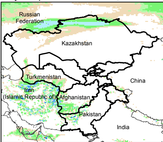
Daily Precip. Forecast for 3 Mar., 2016
