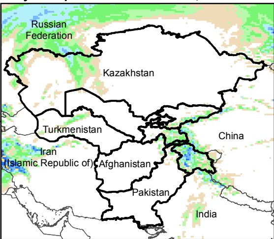
Daily Precip. Forecast for 29 Mar., 2016
