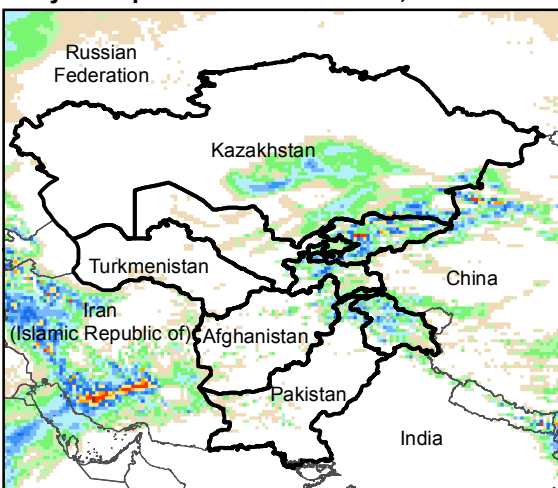
Daily Precip. Forecast for 31 Mar., 2016
