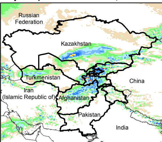
Daily Precip. Forecast for 30 Mar., 2016
