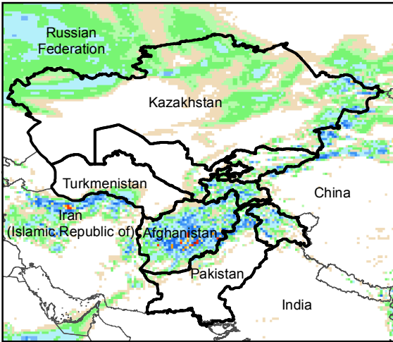
Daily Precip. Forecast for 4 Apr., 2016
