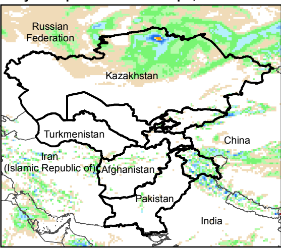
Daily Precip. Forecast for 7 Apr., 2016
