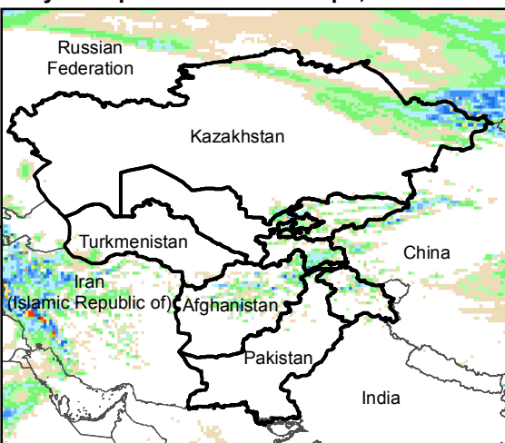
Daily Precip. Forecast for 12 Apr., 2016
