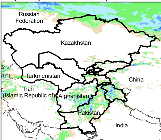
Daily Precip. Forecast for 13 Apr., 2016
