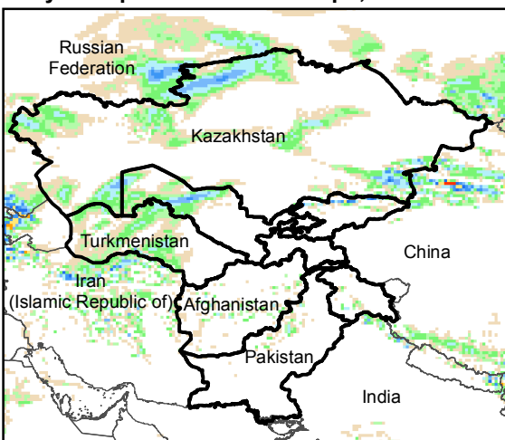
Daily Precip. Forecast for 30 Apr., 2016
