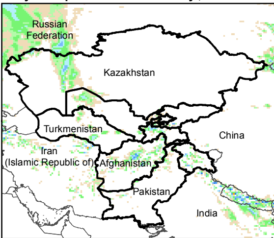
Daily Precip. Forecast for 25 May., 2016
