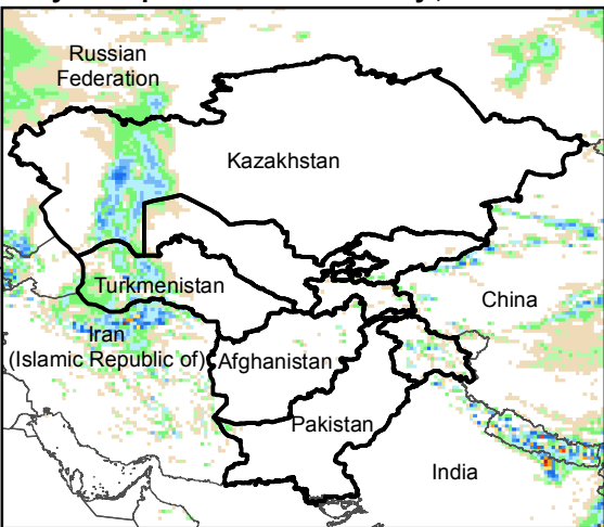
Daily Precip. Forecast for 23 May., 2016
