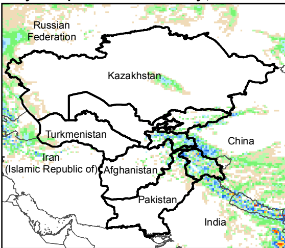
Daily Precip. Forecast for 27 May., 2016
