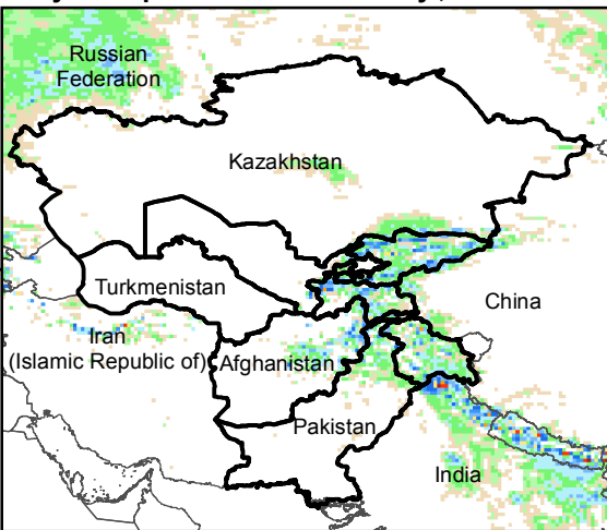
Daily Precip. Forecast for 26 May., 2016
