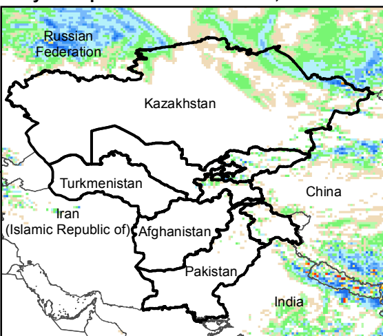
Daily Precip. Forecast for 18 Jun., 2016
