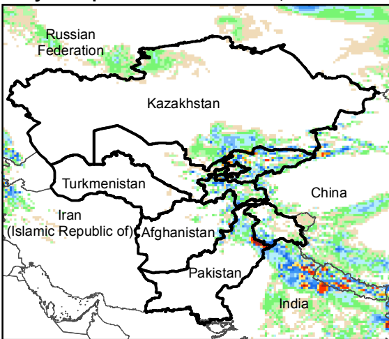
Daily Precip. Forecast for 19 Jun., 2016
