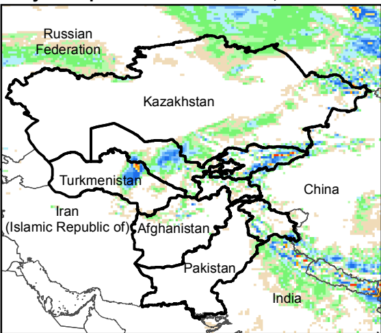
Daily Precip. Forecast for 17 Jun., 2016
