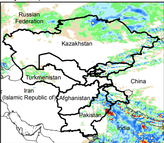
Daily Precip. Forecast for 5 Jul., 2016
