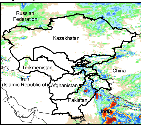
Daily Precip. Forecast for 6 Jul., 2016
