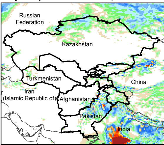
Daily Precip. Forecast for 7 Jul., 2016
