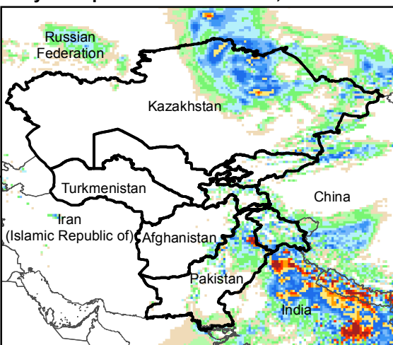
Daily Precip. Forecast for 15 Jul., 2016
