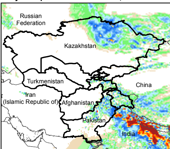
Daily Precip. Forecast for 16 Jul., 2016
