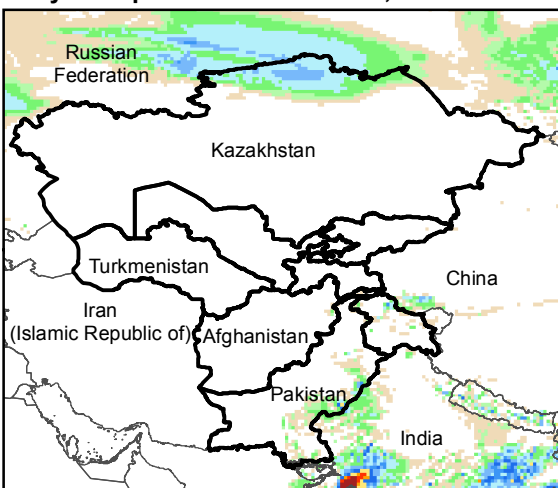
Daily Precip. Forecast for 9 Oct., 2016
