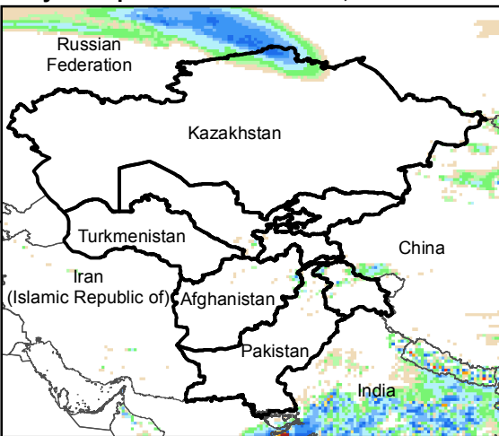
Daily Precip. Forecast for 8 Oct., 2016
