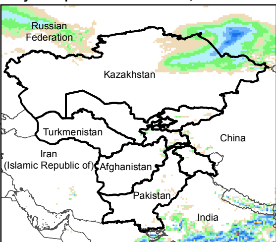
Daily Precip. Forecast for 7 Oct., 2016
