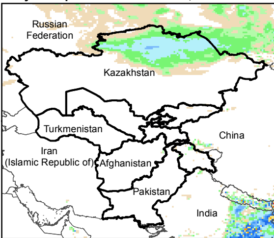
Daily Precip. Forecast for 12 Oct., 2016
