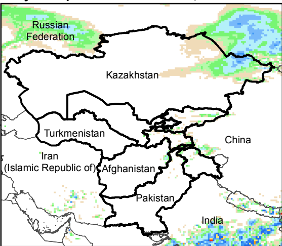
Daily Precip. Forecast for 10 Oct., 2016
