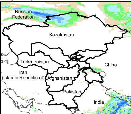
Daily Precip. Forecast for 11 Oct., 2016
