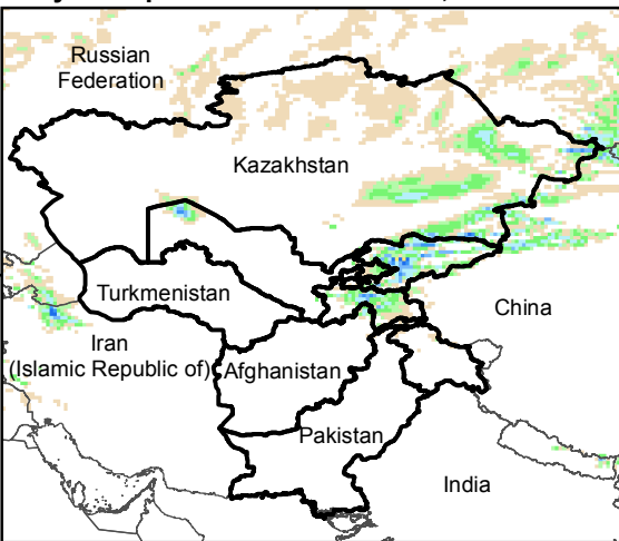
Daily Precip. Forecast for 25 Oct., 2016
