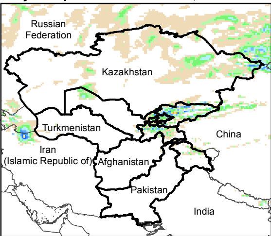
Daily Precip. Forecast for 24 Oct., 2016
