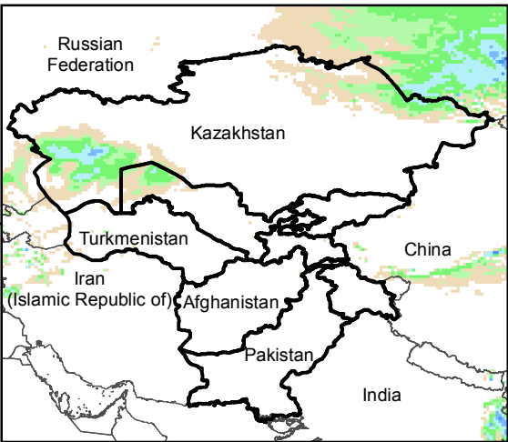
Daily Precip. Forecast for 27 Oct., 2016
