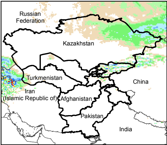
Daily Precip. Forecast for 28 Oct., 2016
