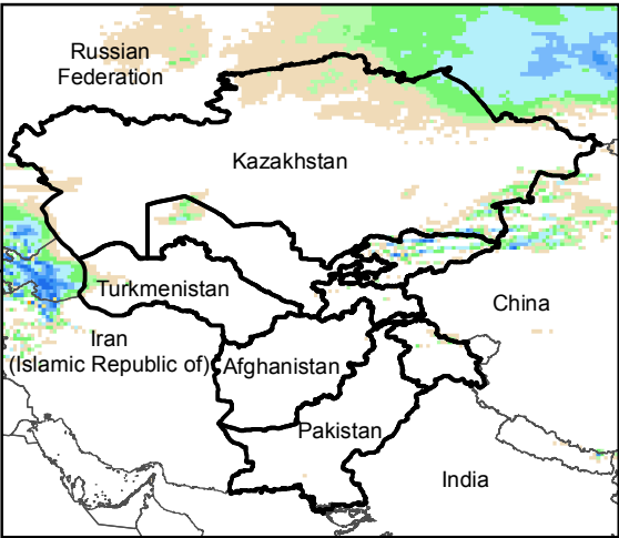
Daily Precip. Forecast for 27 Oct., 2016
