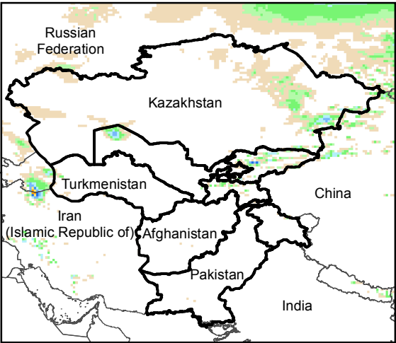
Daily Precip. Forecast for 26 Oct., 2016
