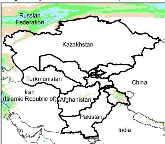
Daily Precip. Forecast for 30 Nov., 2016
