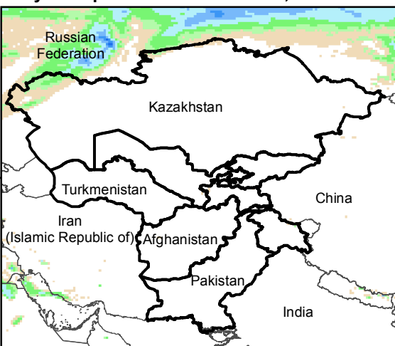
Daily Precip. Forecast for 29 Nov., 2016
