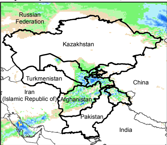
Daily Precip. Forecast for 28 Nov., 2016
