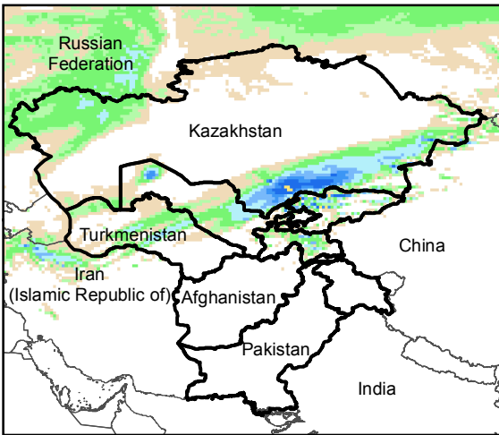
Daily Precip. Forecast for 7 Dec., 2016
