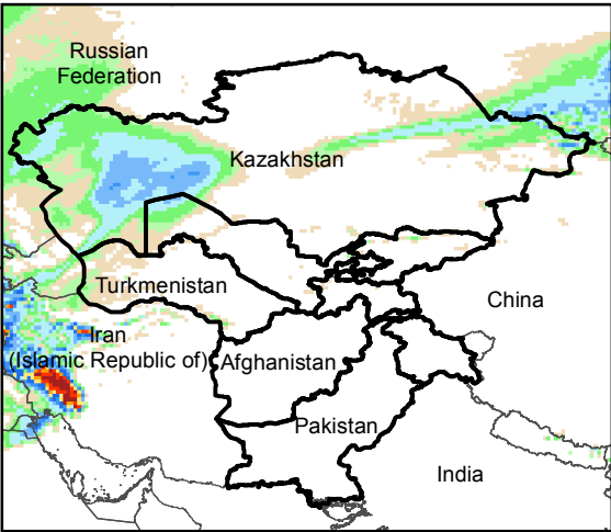
Daily Precip. Forecast for 5 Dec., 2016
