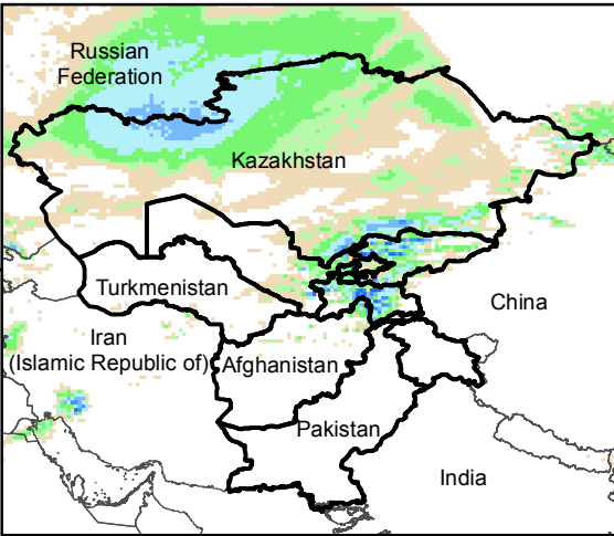
Daily Precip. Forecast for 6 Dec., 2016
