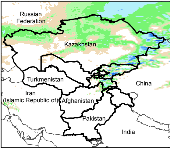
Daily Precip. Forecast for 7 Dec., 2016
