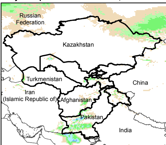
Daily Precip. Forecast for 14 Jan., 2017
