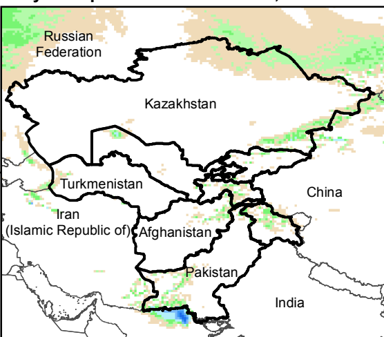
Daily Precip. Forecast for 13 Jan., 2017
