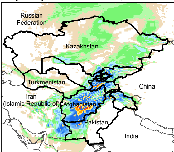
Daily Precip. Forecast for 6 Feb., 2017
