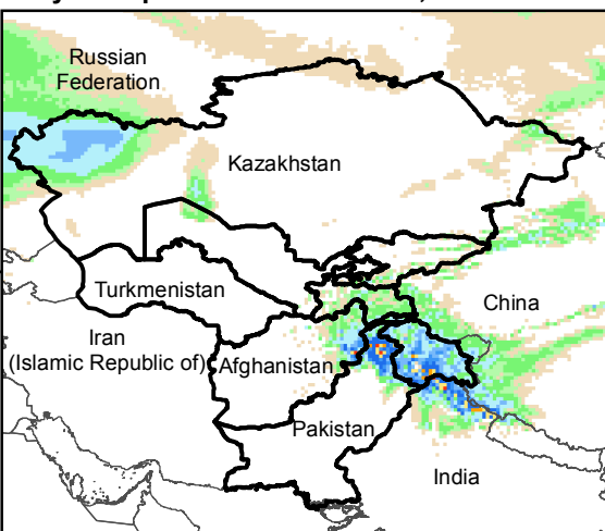
Daily Precip. Forecast for 5 Feb., 2017
