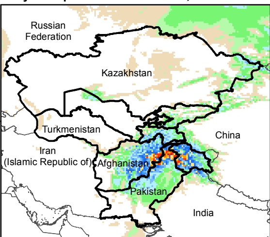
Daily Precip. Forecast for 4 Feb., 2017
