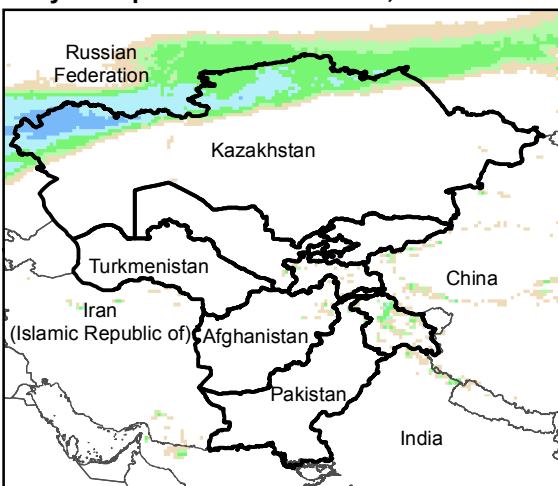
Daily Precip. Forecast for 7 Feb., 2017
